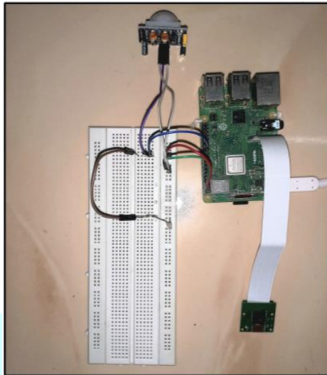
Fig 2. Hardware
