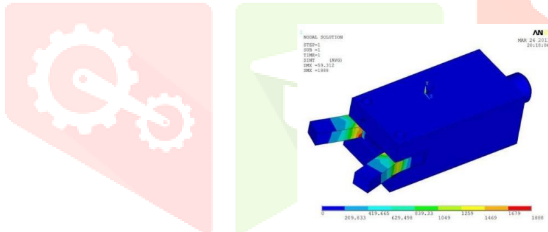
Fig.8 Stress intensity
