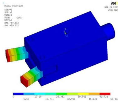
Fig.7 Deformed shape
