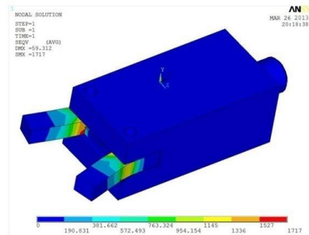
Fig.9 von-mises forces values
