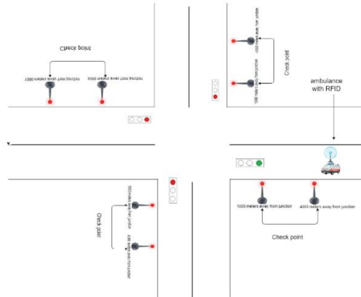
Fig. 3. Traffic Light and Sensors Deployment
