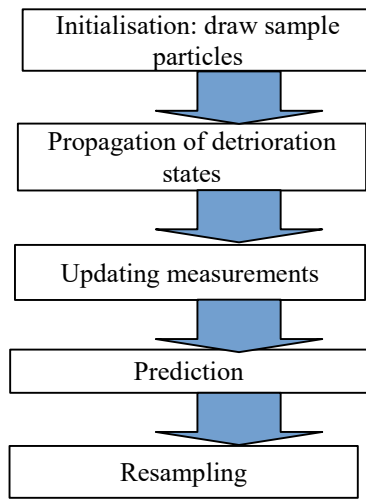
Fig. 1. Flow diagram of particle filtering
