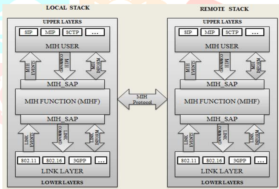
Fig. 4. IEEE 802.21 Media Independent Handover
