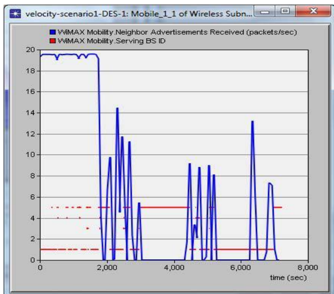
Fig. 9 Handover delay based on IEEE 802.21 MIH standard (Scenario 2)
