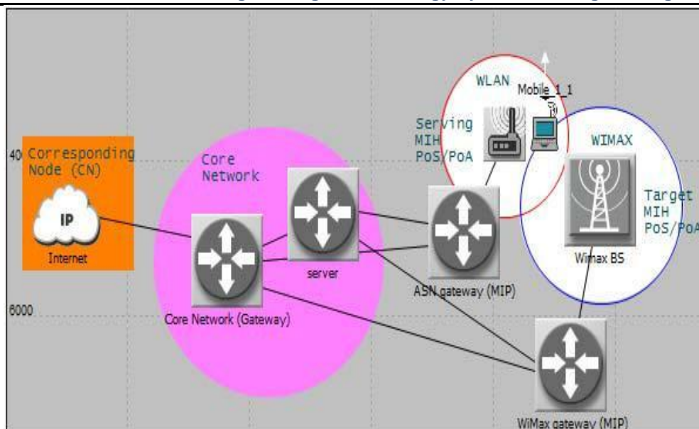
Fig. 6 Vertical Handover between WLAN / WiMAX networks based in IEEE 802.21 MIH standard (Scenario 2)
