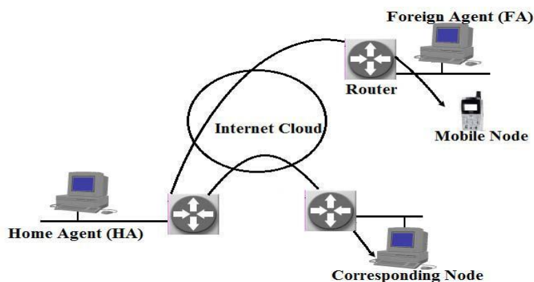
Fig. 3. Mobile IP architecture
