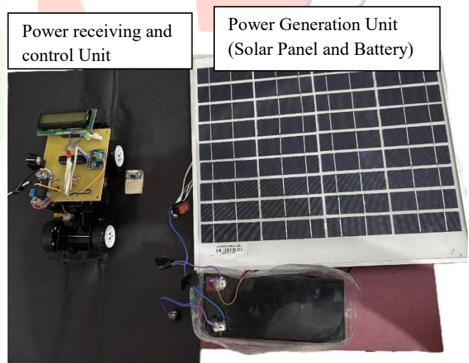
Fig. 3 prototype of DWC System
