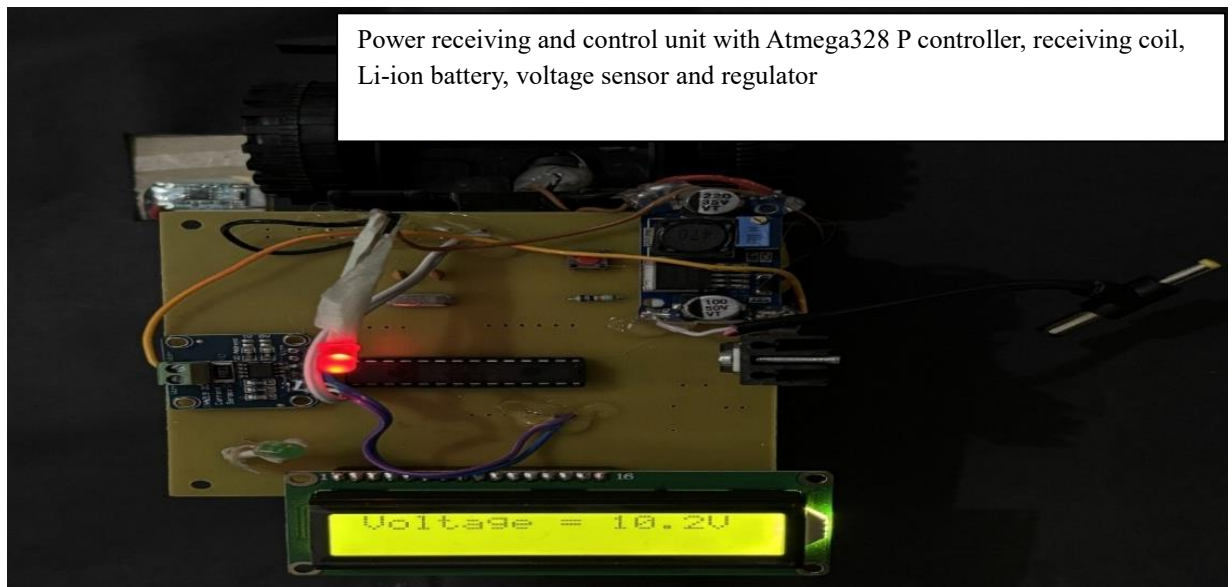
Fig. 4 Power receiving and control unit
