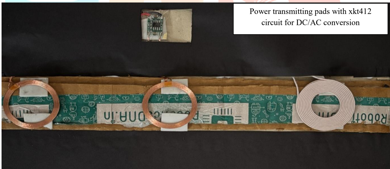
Fig. 5 Power transmitting pads
