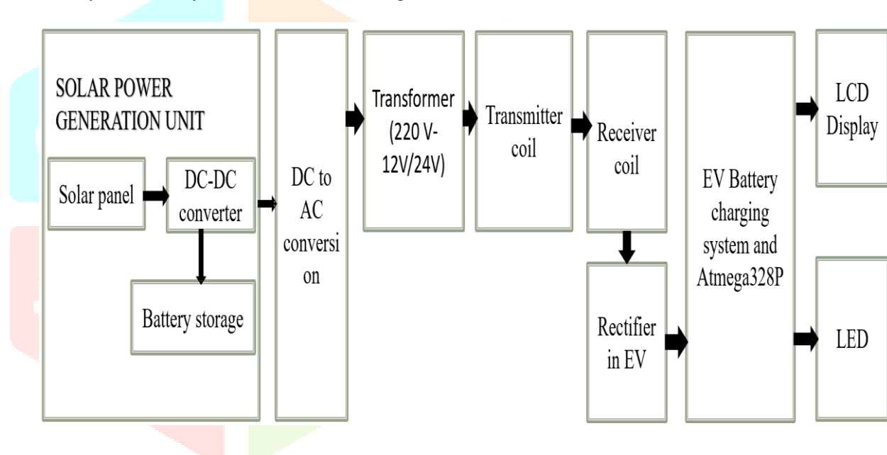
Fig. 1 Block Diagram of Solar Powered Dynamic wireless electric vehicle charging System Using Inductive power transfer Technology
