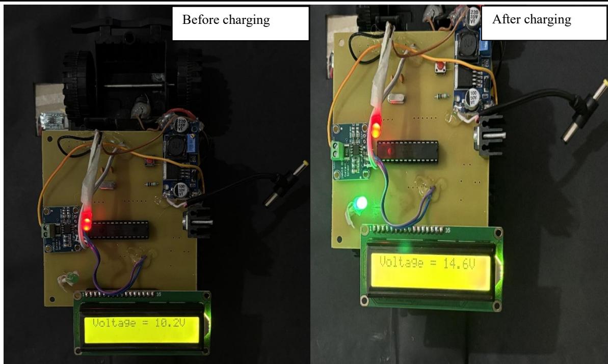
Fig. 6 Display showing before and after charging state of battery
