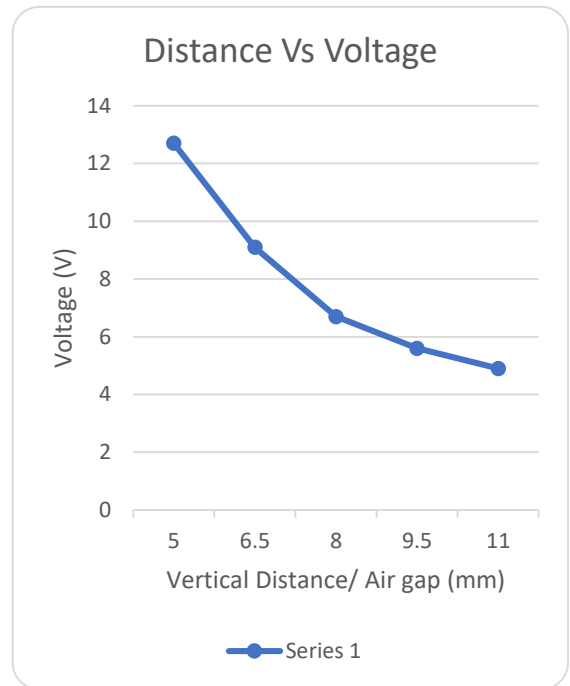
Fig. 2 A Distance (mm) Vs Voltage (V) Graph
