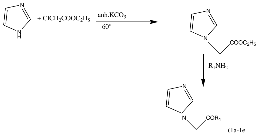
Synthesis of N-substituted imidazole derivatives Figure shows the reaction between imidazole and ethylchloroacetate in the presence of potassium carbonate at 60°. The resulting intermediate (I) reacts with different amines to form the products (1a-1e).
