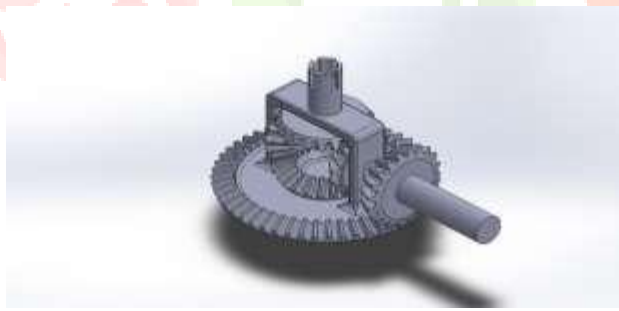
fig 2.5 assembly of differential gearbox
