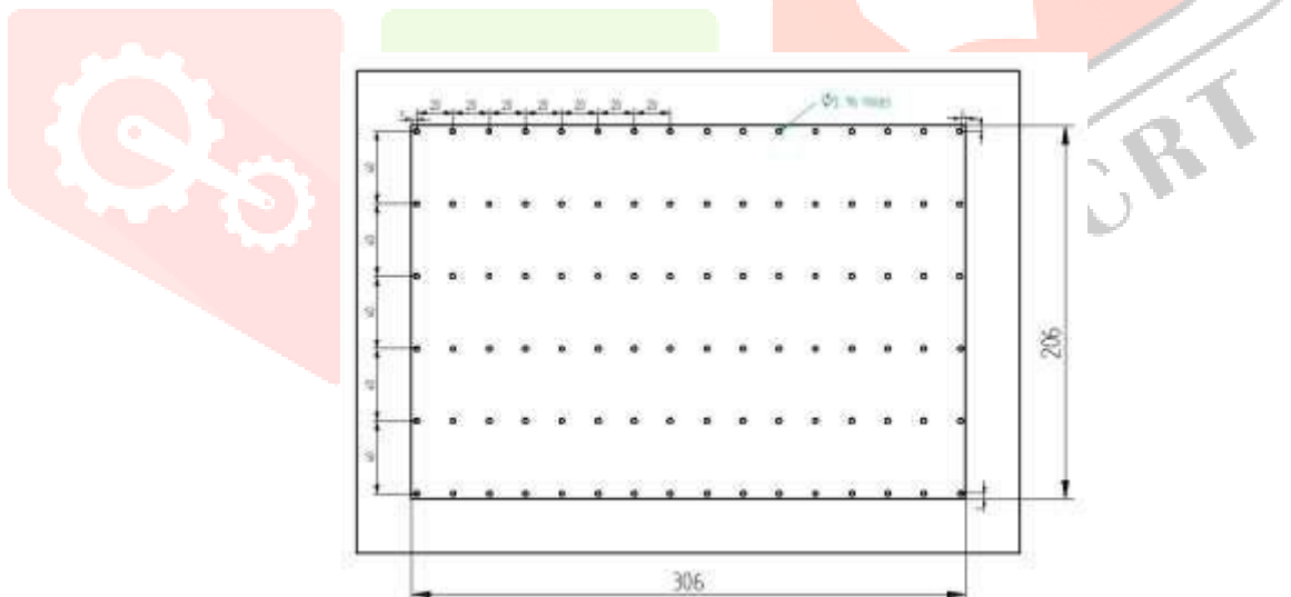
Fig: 2.7: Hole plate draft
