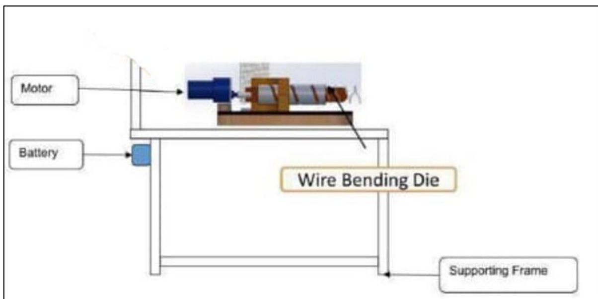
Figure 4.2: Block Diagram of the project HOW DIAMOND MESH CHAIN LINK FENCING IS MADE.
