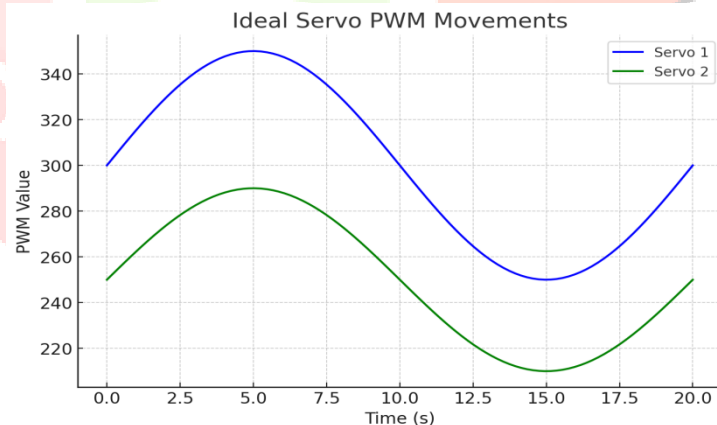
Figure 4.1: Ideal Servo PWM Movements of 2 servos for 20 seconds Interval
