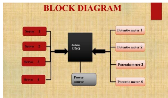
Figure 2.3: Block Diagram of Arduino UNO consists of 4 Servo (SG90) along with Potentiometers and Power Source
