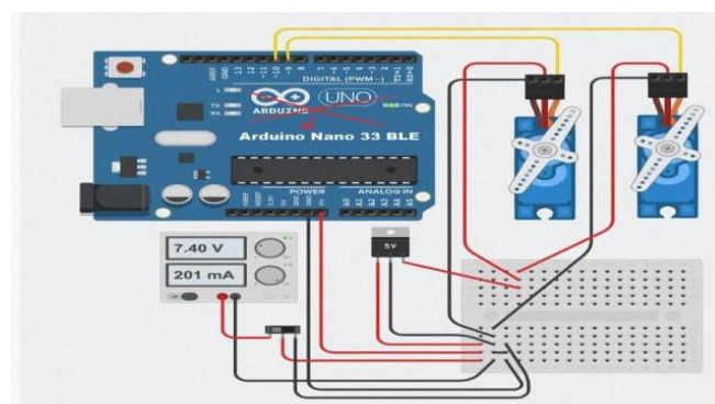
Figure 3.1 Circuit diagram of an experimental setup
