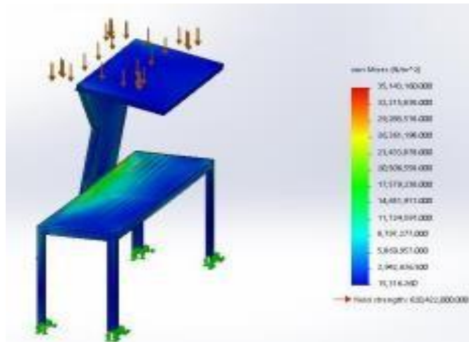
Figure 9-Von Mises for Steel
