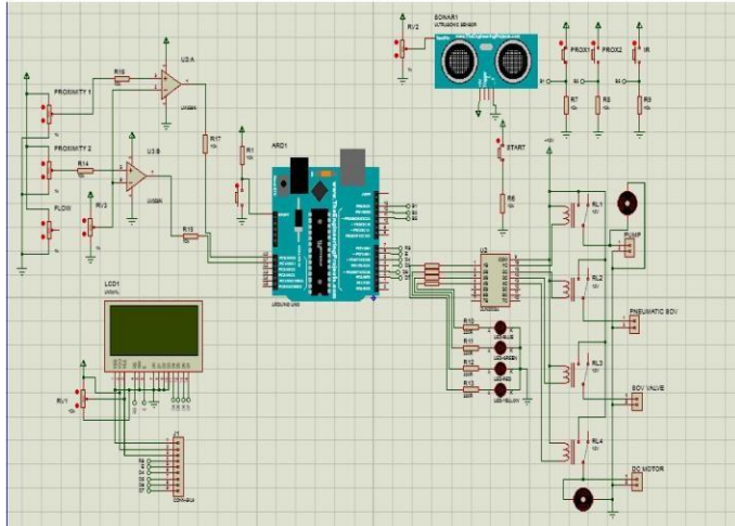
Figure 4-Circuit Schematic
