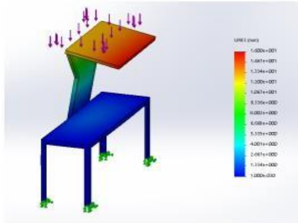
Figure 6-Aluminium 1060 under deflection
