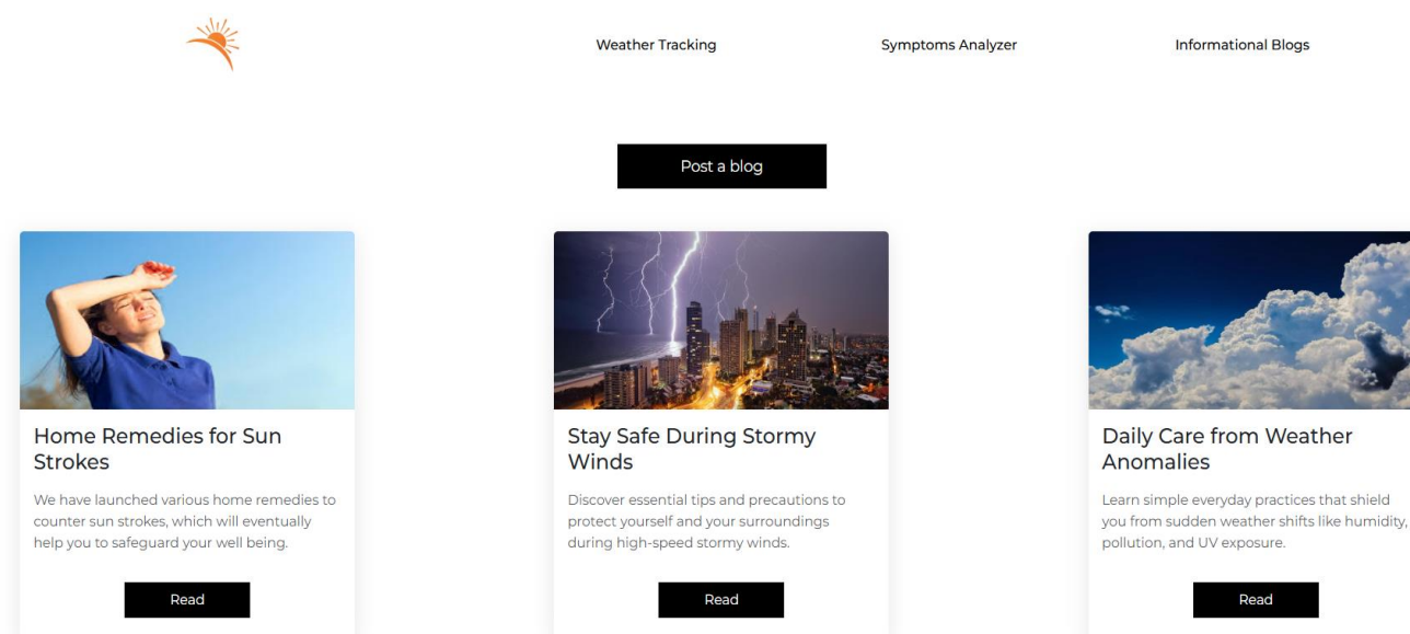
Fig. 6.3. Blogs
