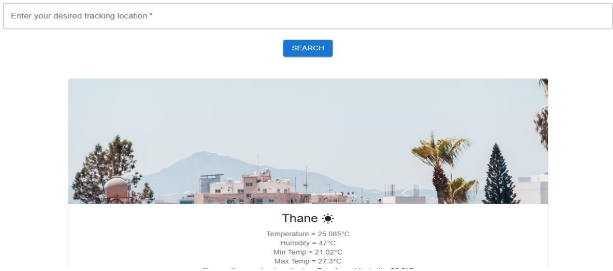
Fig. 6.1. Weather Tracking
