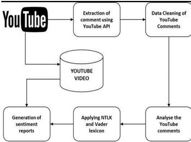
FIGUREI System Architecture
