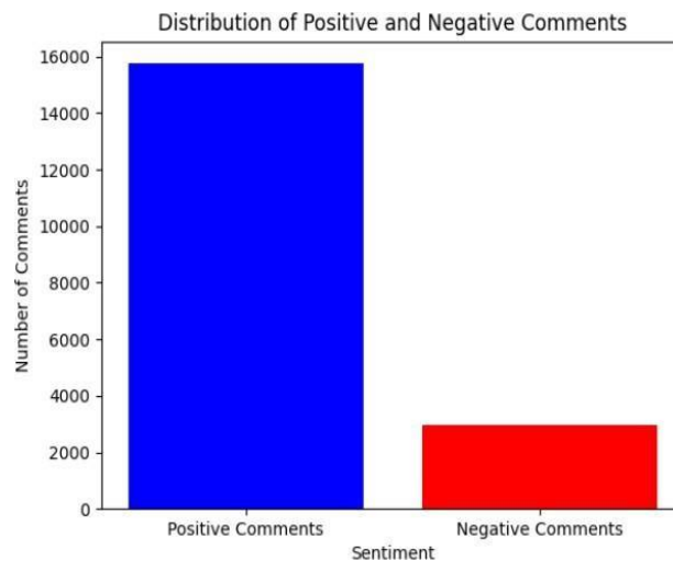
FIGUREIII Bar Graph
