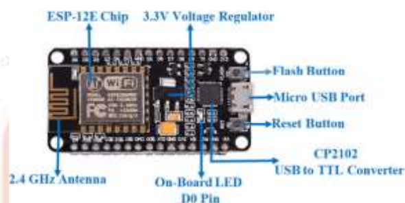
Fig. 2 NodeMCU Development Kit
