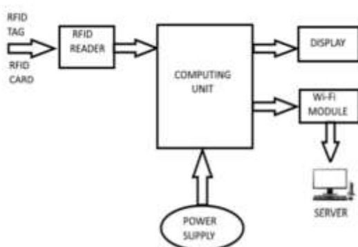
Fig. 1 Block Diagram
