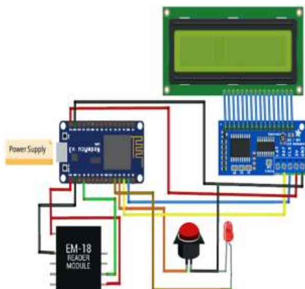
Fig. 7 Circuit Diagram
