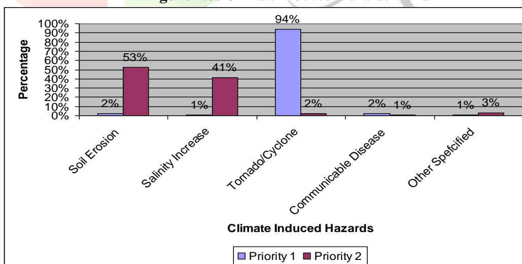
Figure 4.8: Climate Induced Hazards
