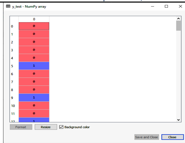
Figure 4: Y test
