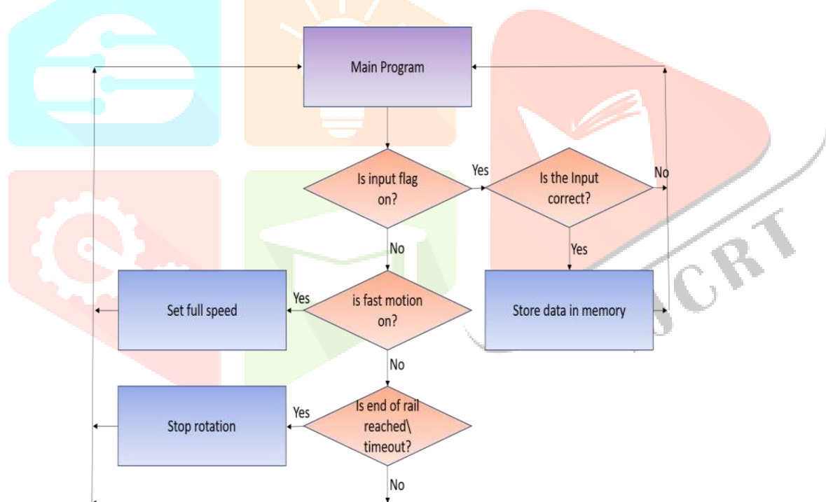
Fig.2. Flowchart of the algorithm to control the motion of the crystal inside the furnace
