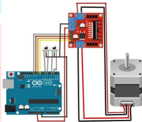
Fig.3. Arduino box and schematics drawn with Fritzing [8]
