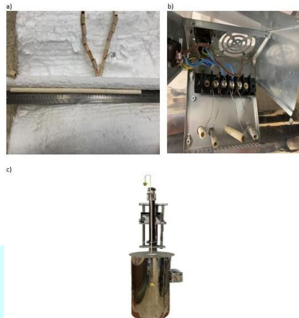
Fig.5. Assembly of Bridgman method furnace. a) Heating wires wrapped around 2.5 [mm] X 70 [cm] ceramic tube. b) The heating wires connection to the power box. c) The fully assembled system, the furnace at the bottom and translation stage above it
